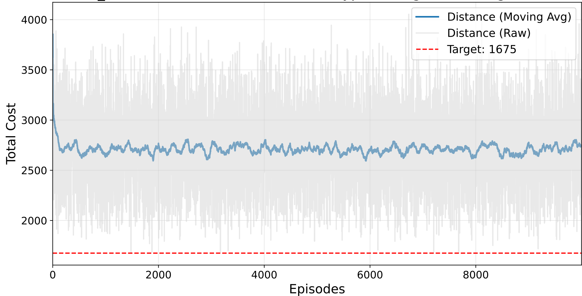
Final NO_BAYESIAN Masked AutoRL-SOP (HyperTuningSK) Training - ESC12.sop
